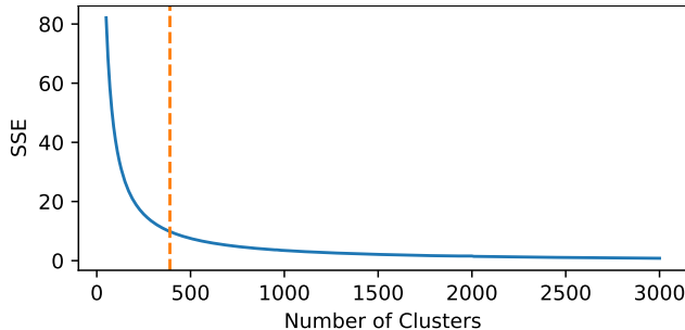
Fig. 2. Sum of squared errors using the distances between comments for different number of clusters (the dashed line depicts the elbow of the curve)
