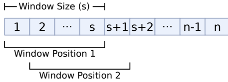
Figure 3: Sliding Window Technique
